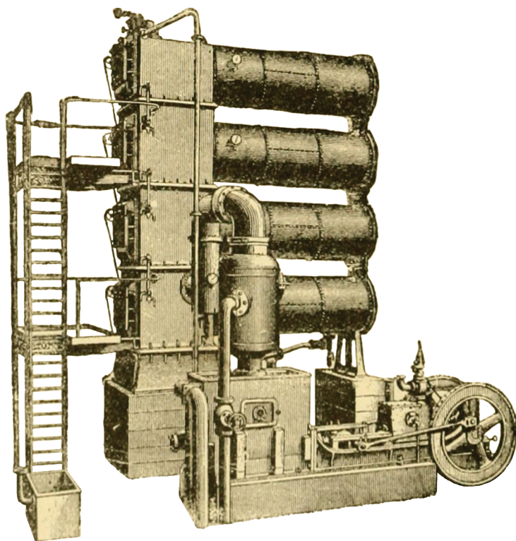
Multiple-effect evaporator
